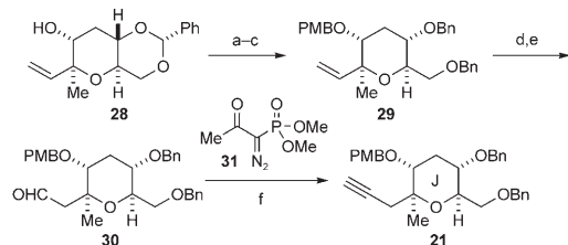
Scheme 5. Reagents and conditions: a) NaH, PMBCl, TBAI, DMF, 0°C→RT; b) CSA, MeOH, 0°C→RT, 86% (2 steps); c) NaH, BnBr, TBAI, DMF, 0°C→RT, 94%; d) 9-BBN, THF, 0°C→RT; aq NaOH, H 2 O 2 , 0°C→RT, 71%; e) TPAP, NMO, 4-Å MS, CH 2 Cl 2 , 0°C→RT, 77%; f) Cs 2 CO 3 , i PrOH, 0°C→RT, 93%. PMB = p -methoxybenzyl.
